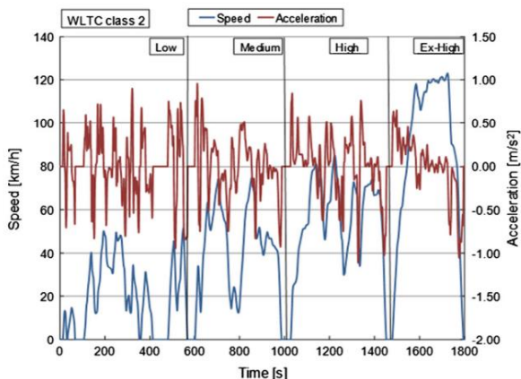
Figure 3. WLTC Class 2 v3.2 Speed and acceleration profiles.
